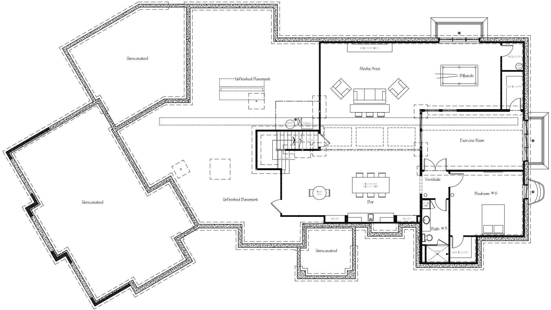
Finished Lower Level Plan Scale: 1/8" = 1'-0"
